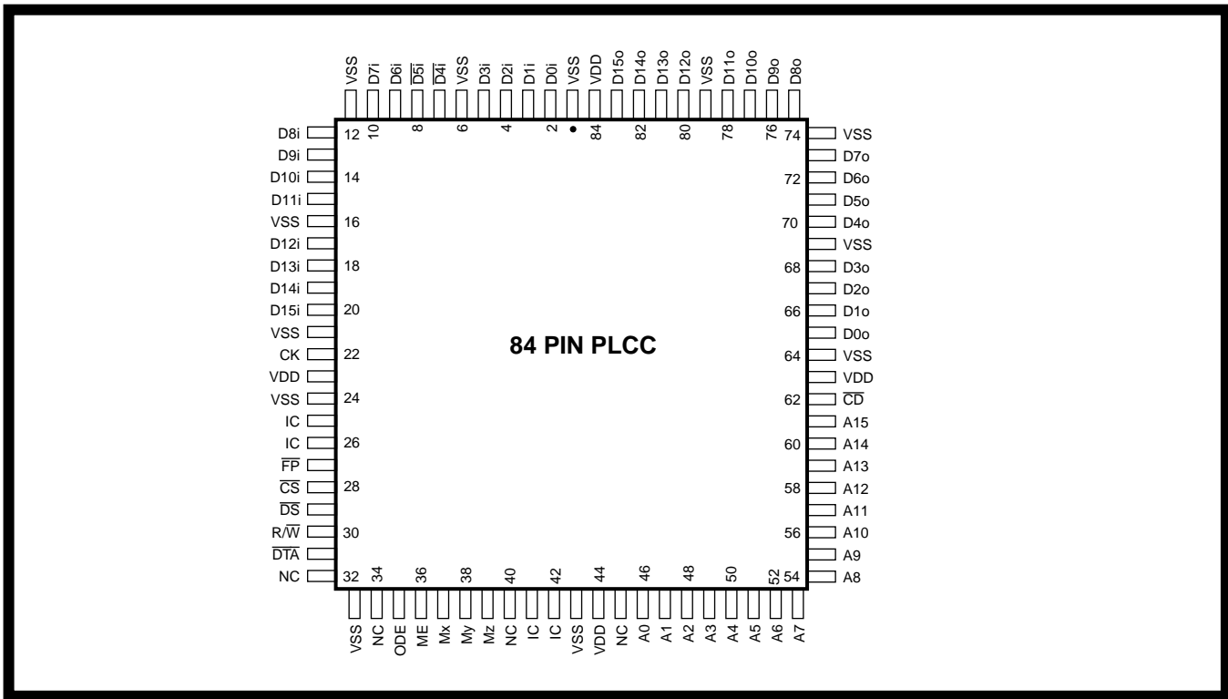
Figure 2 - Pin Connections
